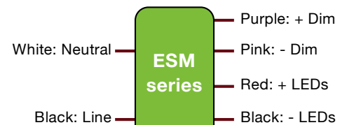
Wiring Diagram
